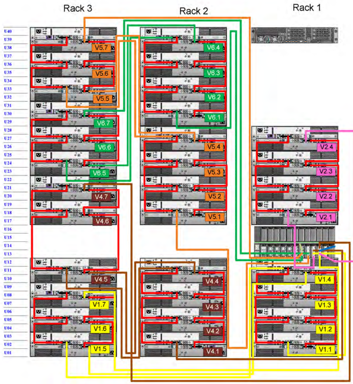
Figure 54. Recommended cabling for DD4500 with extended retention and integrated with Avamar
