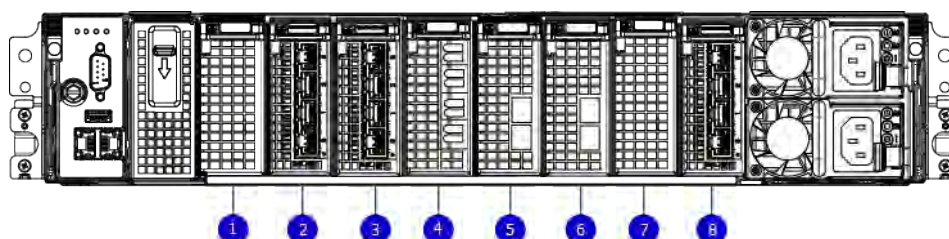
Figure 75. I/O module slot numbering
