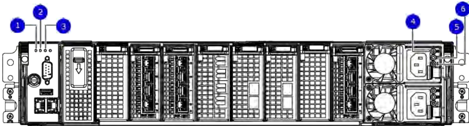
Figure 72. Rear LED indicators
