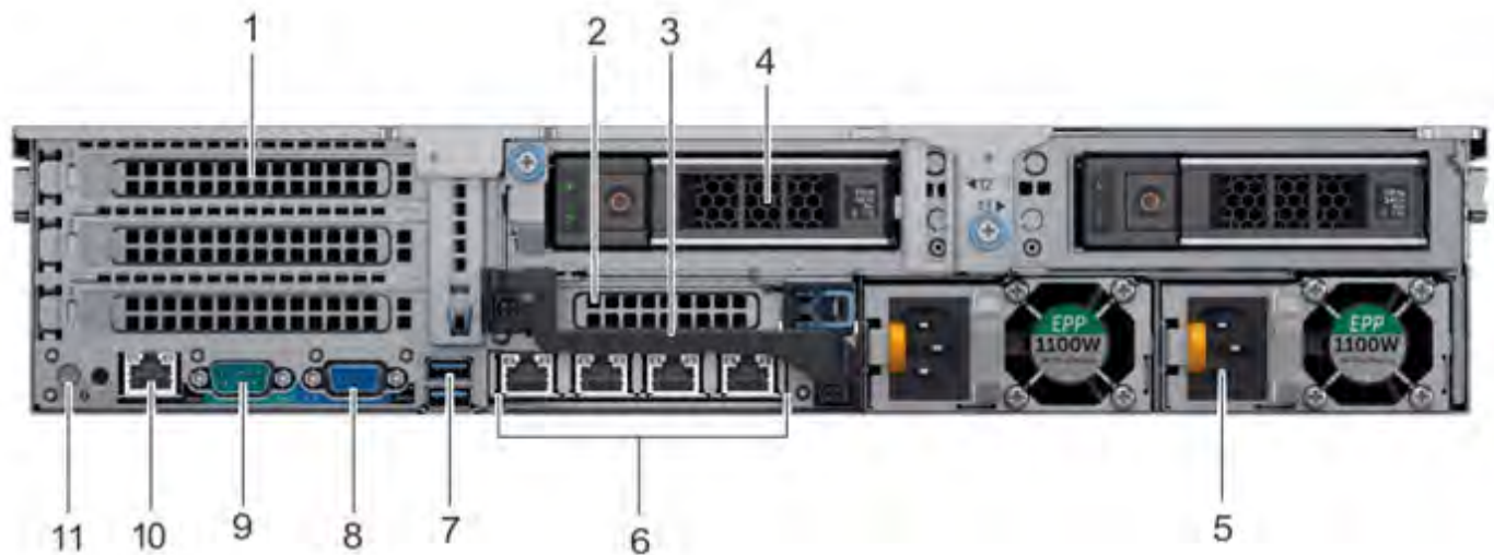
Figure 6. Rear panel
