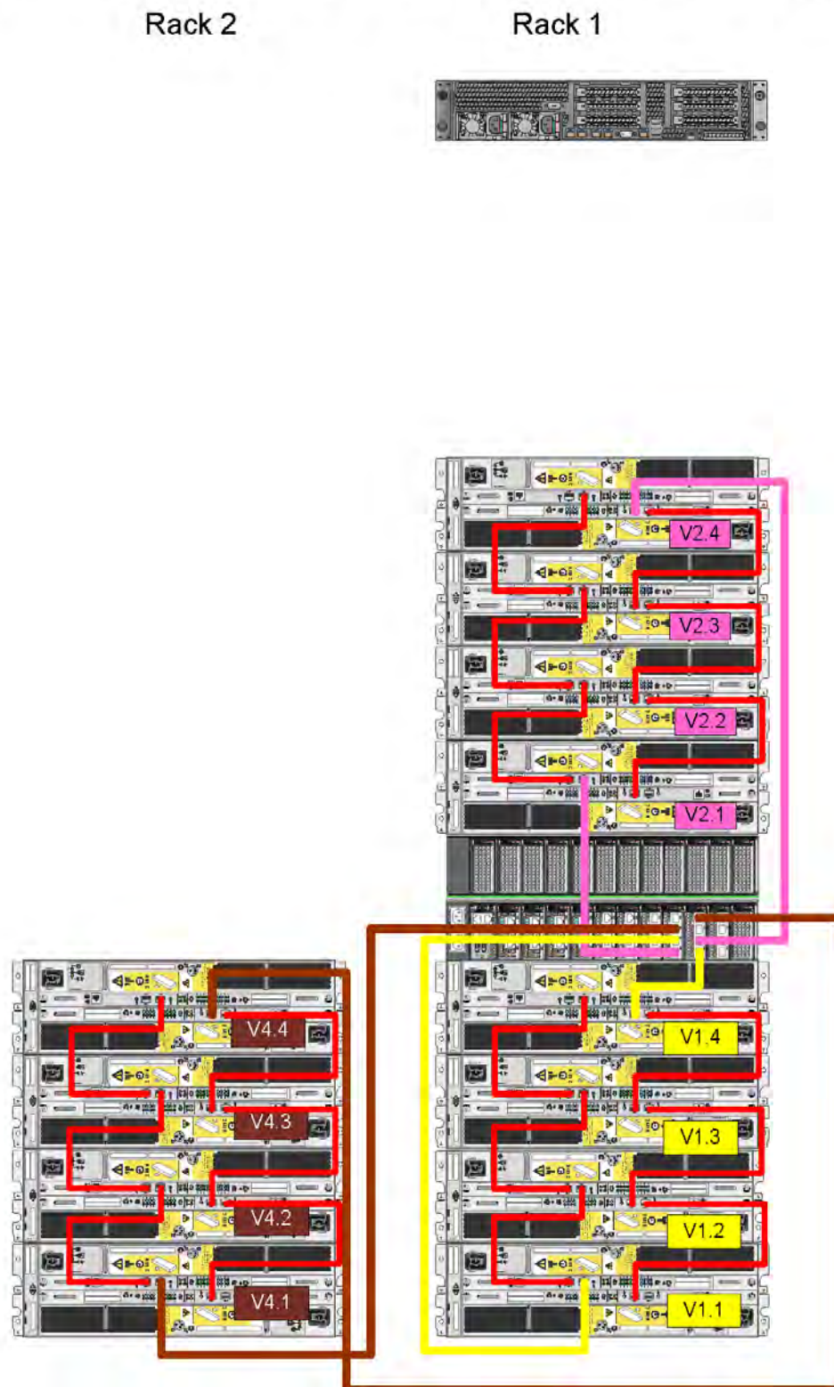
Figure 52. Recommended cabling for DD4500 integrated with Avamar
