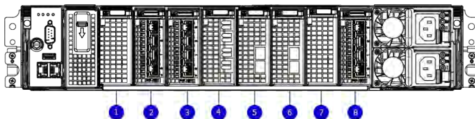
Figure 69. I/O module slot numbering
