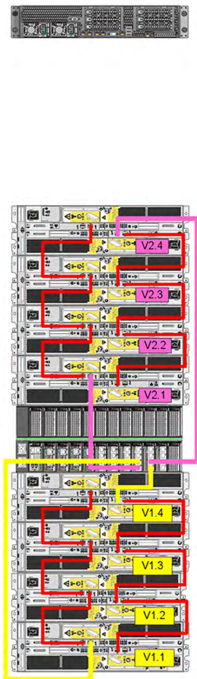
Figure 32. Recommended cabling for DD4200 integrated with Avamar
