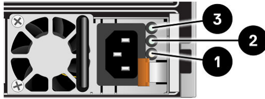
Figure 16. NVMe expansion enclosure AC power supply LEDs
