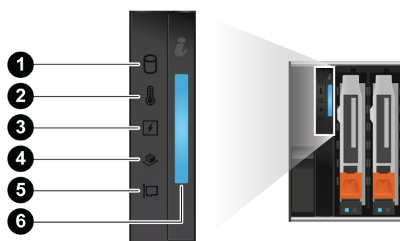
Figure 12. NVMe expansion enclosure status LEDs
